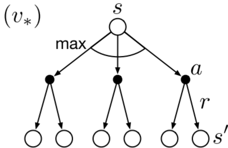
Backup diagrams for v^* and q^*
